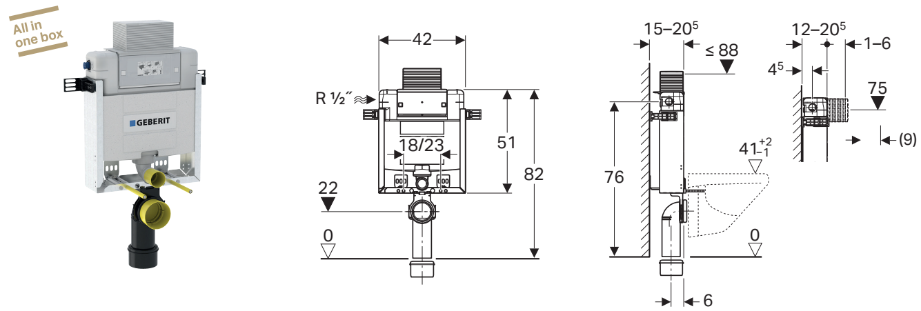
Geberit Alpha Kombifix, low height 12 cm, top / front operated 6/3L flush.
