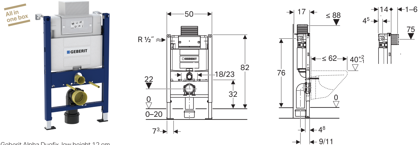
Geberit Alpha Duofix, low height 12 cm, top / front operated 6/3L flush.
